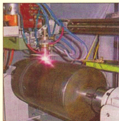
Fig. 1 — Plasma arc welding with powder containing an extremely high share of carbides.
