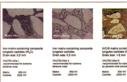
Fig. 6 — Welding fillers containing tungsten carbides.
